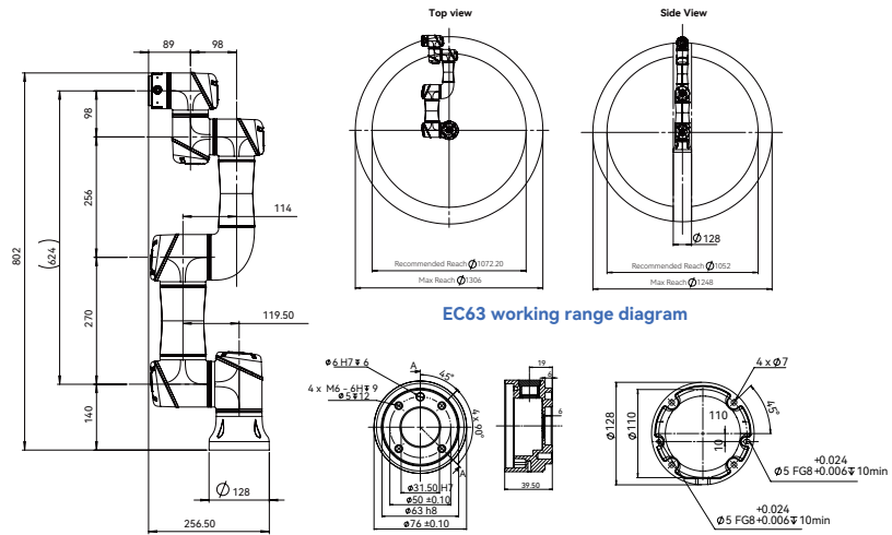
EC63 external dimensional drawing
